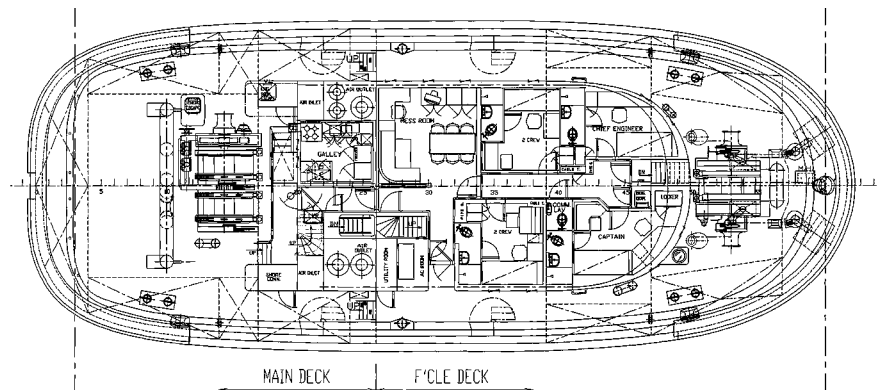
MAIN DECK
