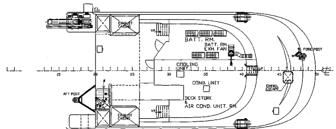
DECKHOUSE DECK
