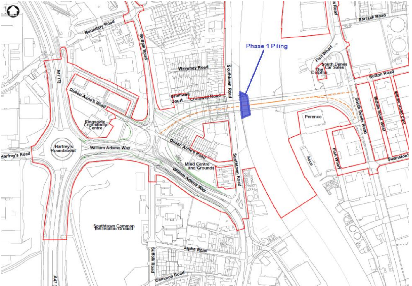
Fig. 2 – Bridge Structure Outline and Phase 1 Piling Location
