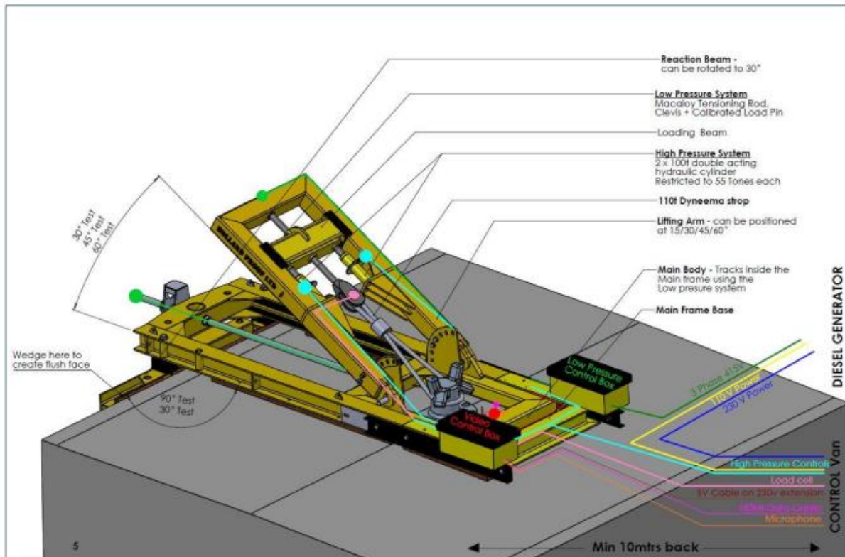
Fig 1 – Test Rig
