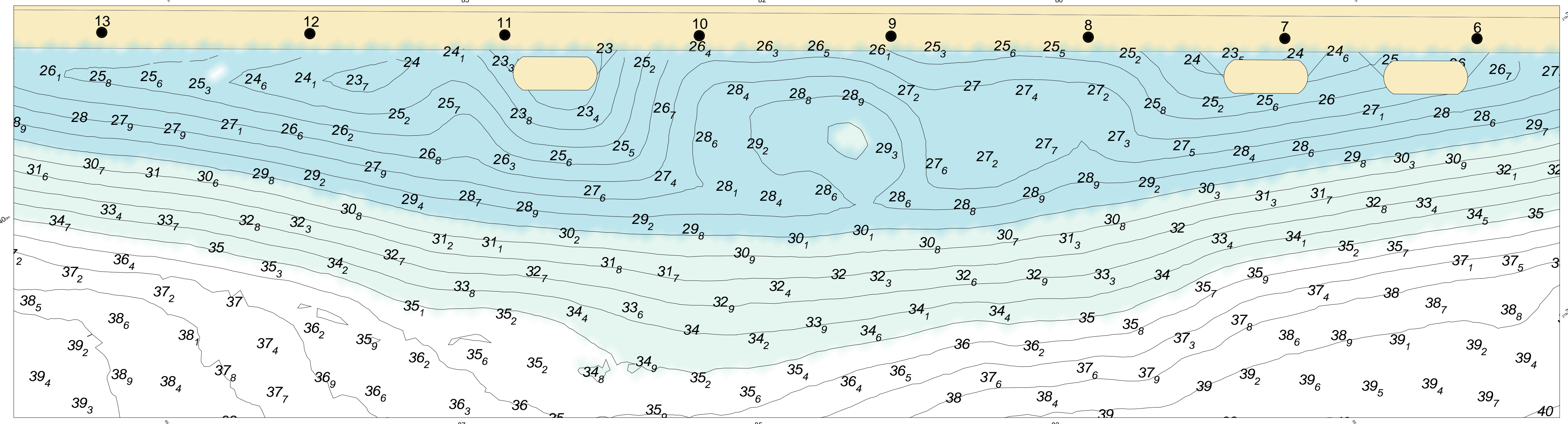
Outer Jetty Bollards 6 to 13 at 1:250 scale showing Coal Build-up.
